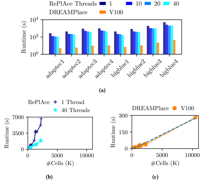
Figure 5: (a) GP runtime for ISPD 2005 benchmarks. (b) GP runtime scaling for RePlace on ISPD and industrial benchmarks. The points for the 10-million-cell benchmark design6 are omitted due to crash. (c) GP runtime scaling for DREAMPlace.
